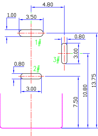
RECOMMENDED PCB LAYOUT TOP VIEW TOLERANCE: \pm 0.05
