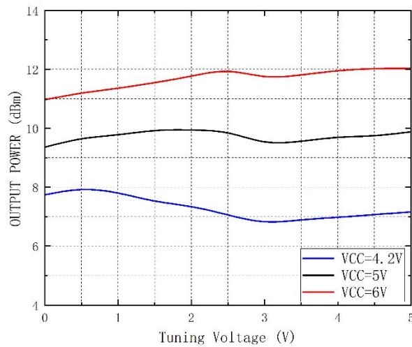
Power vs. Tuning Voltage vs. Operating Voltage
