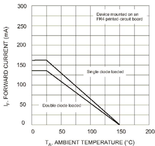
Fig. 2 Current Derating Curve
