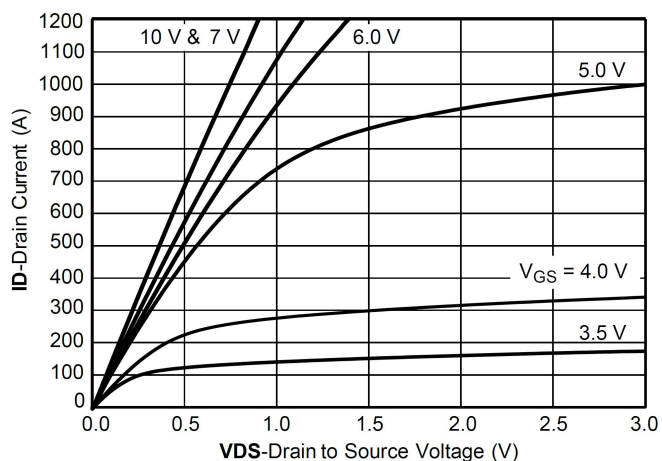
Output Characteristics
