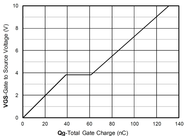
Gate Charge
