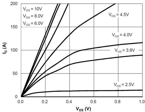
Saturation Characteristics
