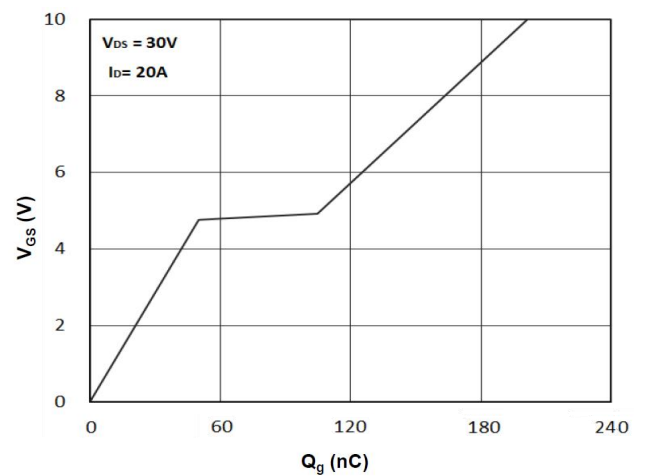
Gate Charge
