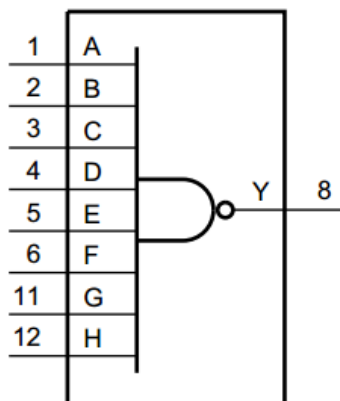
Figure 1. Logic symbol
