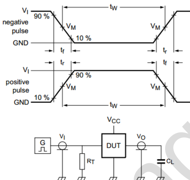
Figure 4. Test circuit for measuring switching times
