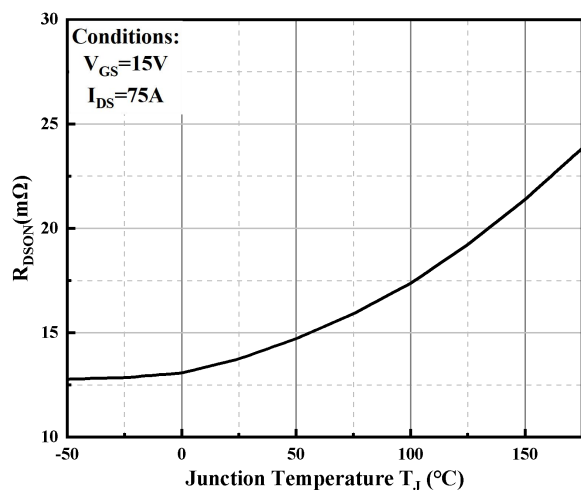
Normalized On-Resistance with Temperature
