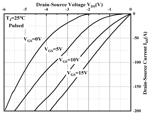
Drain-Source Current vs Drain-Source Voltage(25°C)
