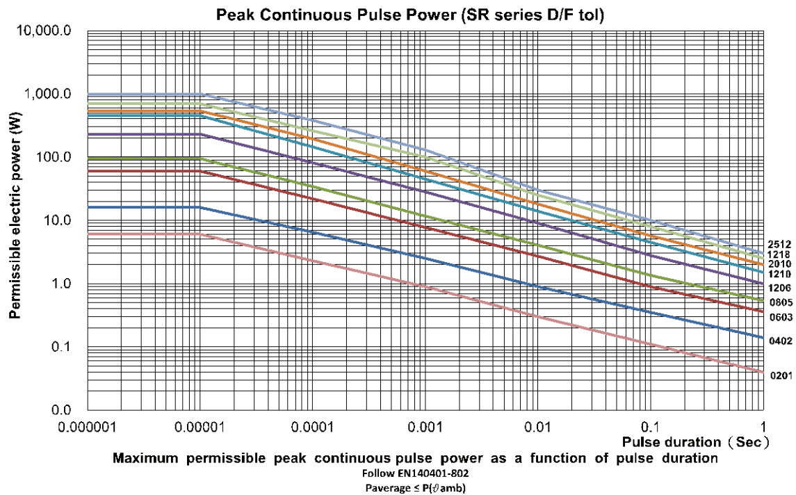
Fig. 7-3 Pulse-Load behavior
