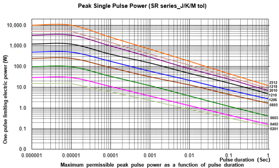
Fig. 7-2 Pulse-Load behavior
