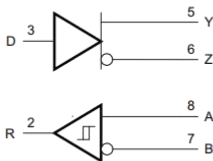
Figure 16. SN65HVD17xx Always-Enabled Driver Receiver
