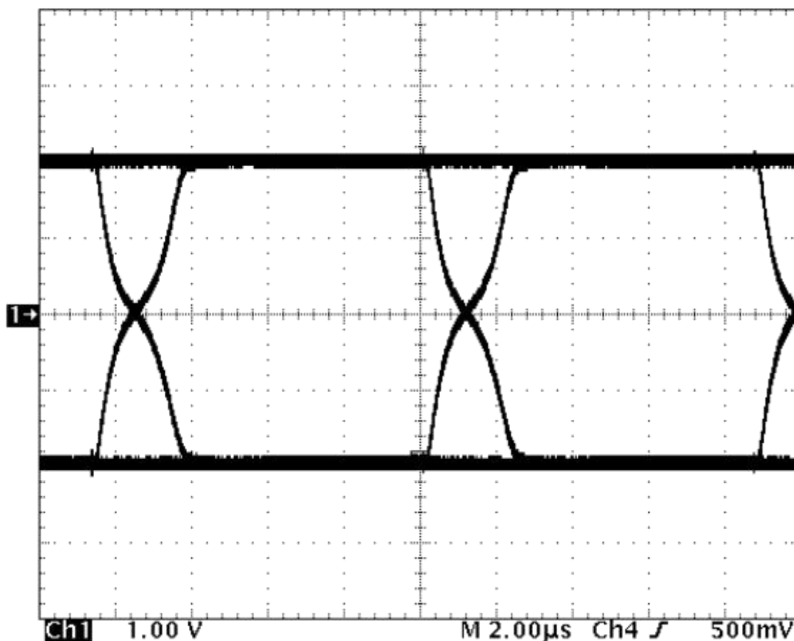
Figure 21. SN65HVD1785 Differential Output at 115 kbps
