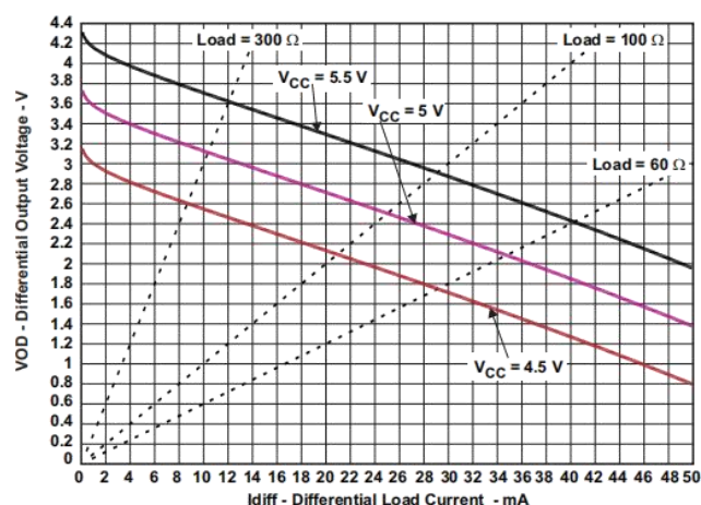
Figure 4. Differential Output Voltage vs. Differential Load Current
