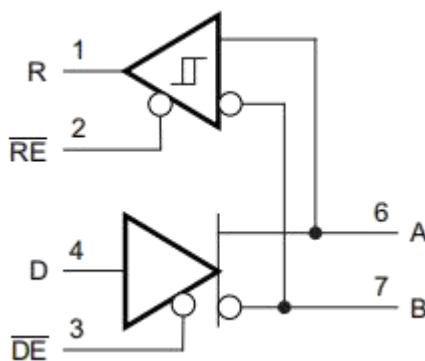
Figure 15. SN65HVD1708E Transceiver for J1708 Applications
