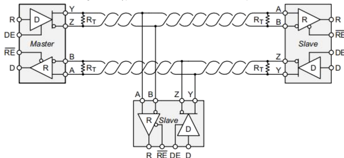
Figure 19. Typical RS-485 Network With Full-duplex Transceivers
