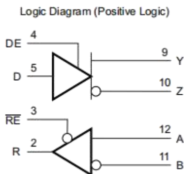
Figure 14. Full Duplex Transceiver
