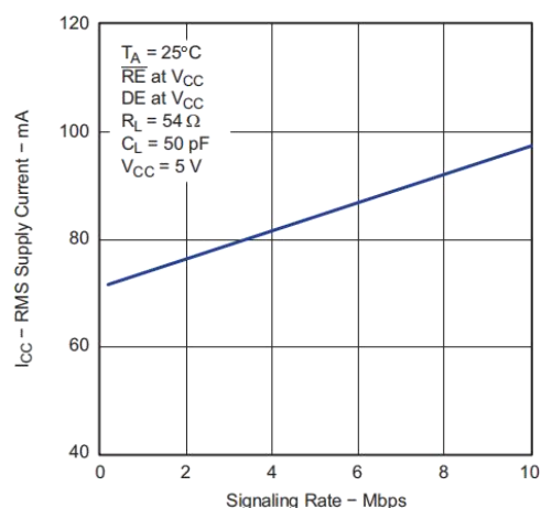
Figure 2. HVD1787 RMS Supply Current vs Signaling Rate
