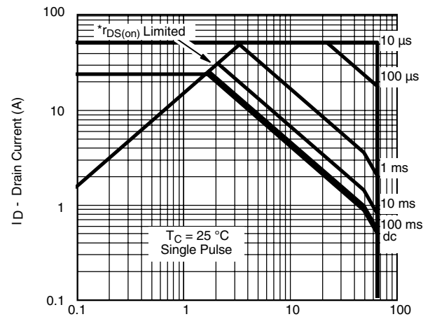
V_{DS} - Drain-to-Source Voltage (V) *V_{GS} > \text{minimum } V_{GS} \text{ at which } r_{DS(on)} \text{ is specified} Safe Operating Area
