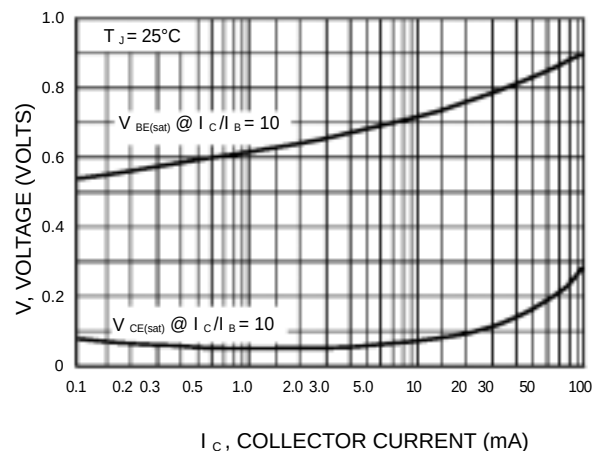
Figure 4. "On" Voltages
