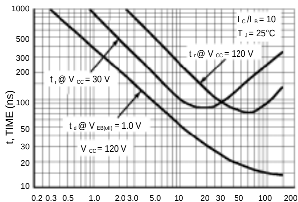
8. Turn-On Time
