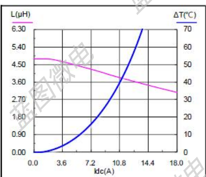
SMS1050-4R7M
