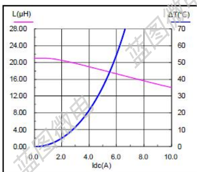
SMS1050-220M
