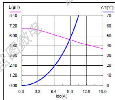
SMS1050-6R8M
