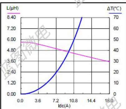
SMS1050-5R6M
