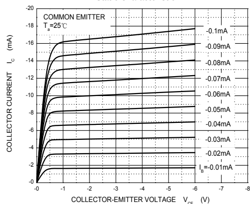
Static Characteristic
