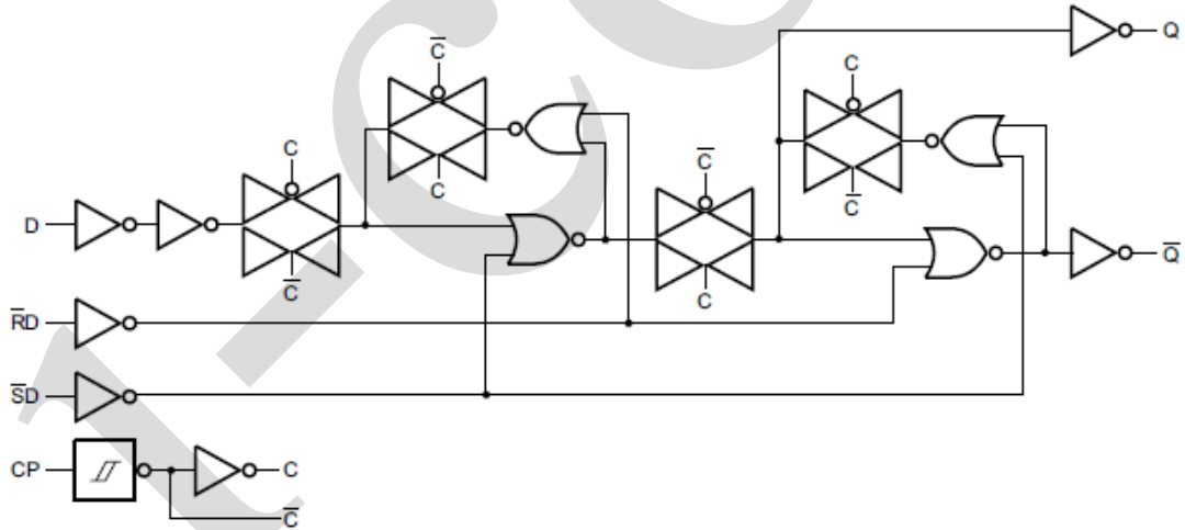
Figure 3. Logic diagram
