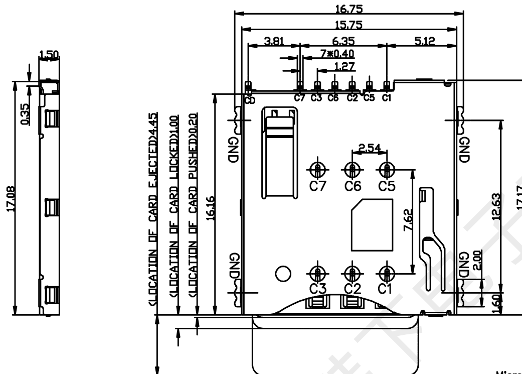
MicroSIM CARD
