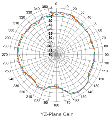
Figure 7. ANT-DB1-nSP250 Antenna Radiation Patterns
