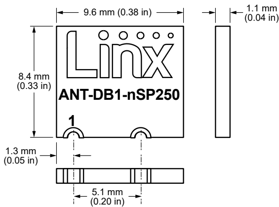
Figure 1. ANT-DB1-nSP250 Antenna Dimensions
