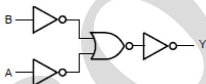
Figure 3. Logic diagram
