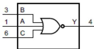
Figure 1. Logic symbol
