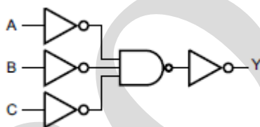
Figure 3. Logic diagram
