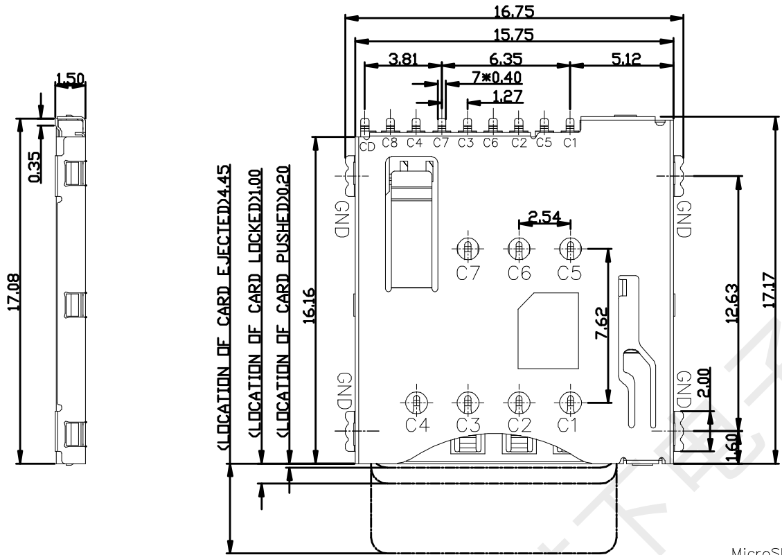
MicroSIM CARD
