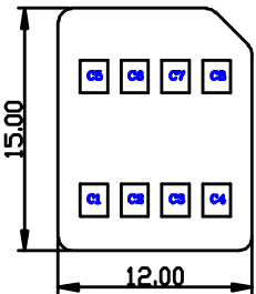
MicroSIM CARD
