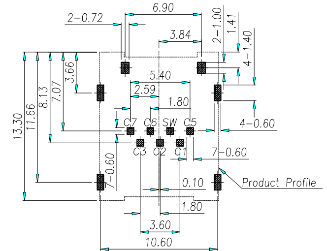
RECOMMENDED PCB LAYOUT GENERAL TOLERANCE (.XX±0.05)
