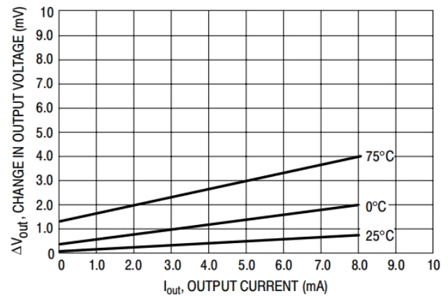
Figure 4. Change in Output Voltage v versus Load Current (Normalized to V_{out} @ V_{in} = 15\text{ V} , I_{out} = 0\text{ mA} )
