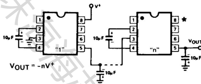
Figure 5. Cascading ICL7662CPA-HX for Increased Output Voltage
