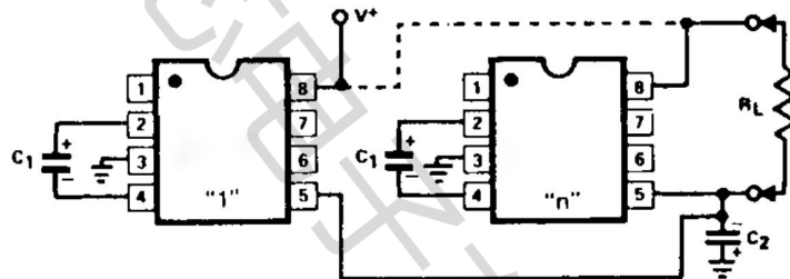
Figure 8. Paralleling ICL7662CPA-HXs to Reduce Output Resistance
