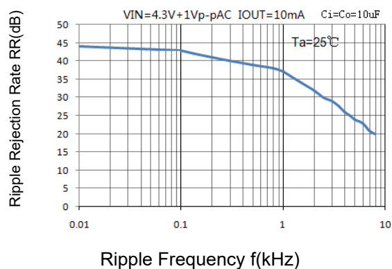
Figure 5: Ripple suppression
