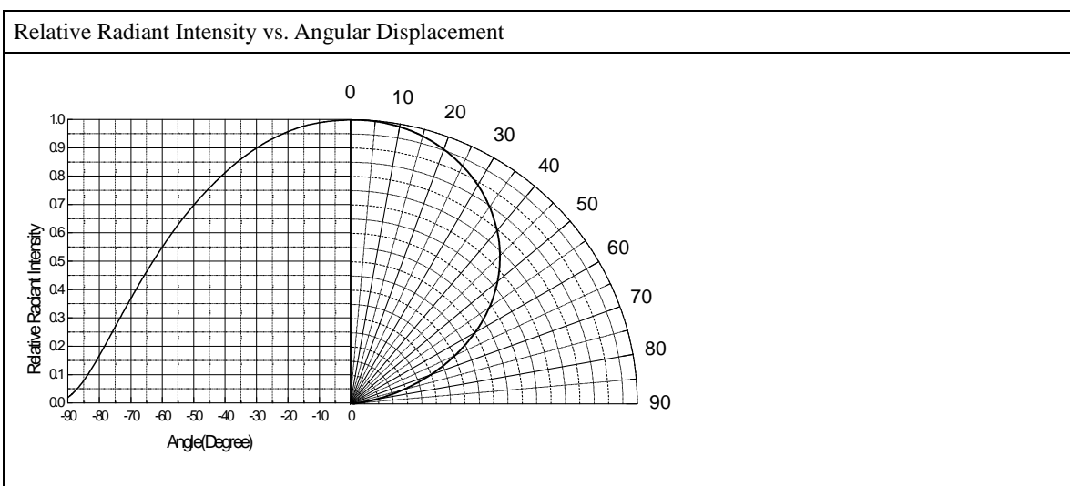
Typical Electrical/Optical/Characteristics Curves
