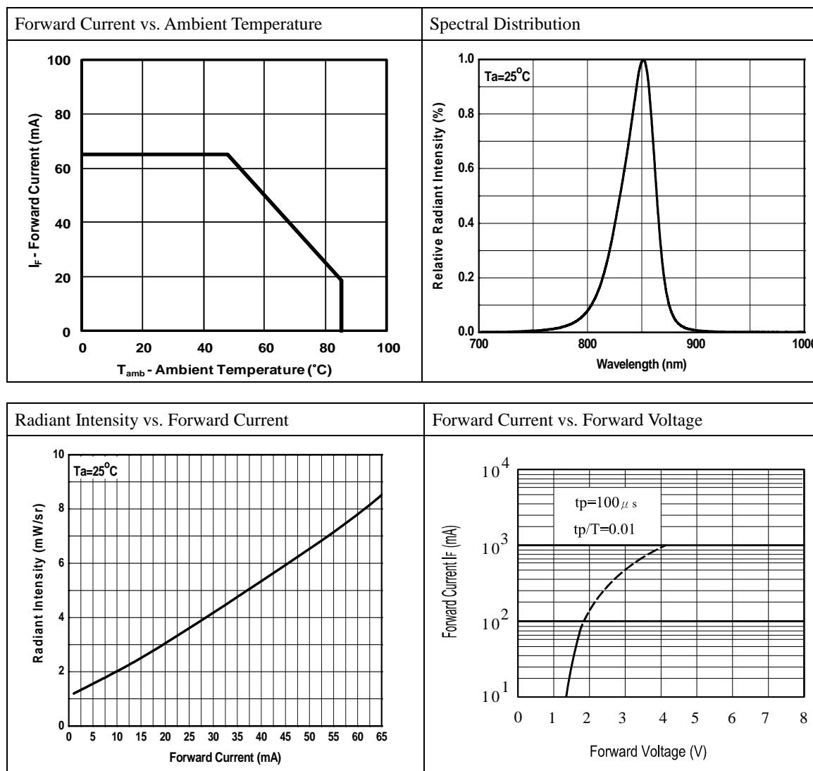
Typical Electrical/Optical/Characteristics Curves
