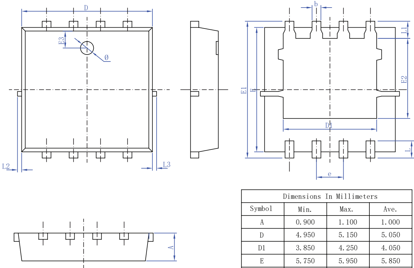
DFN-8 5x6
