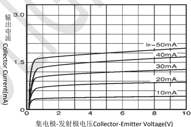
Output Characteristics
