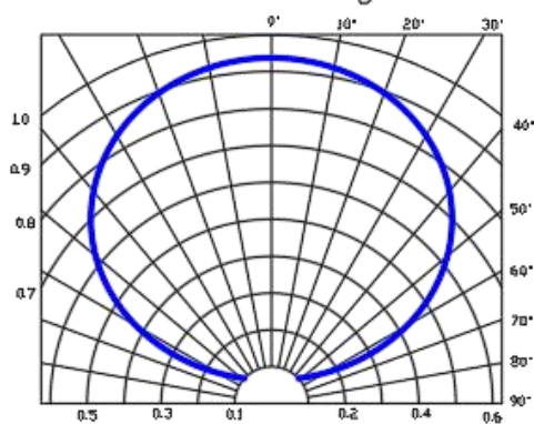
Radiation angle
