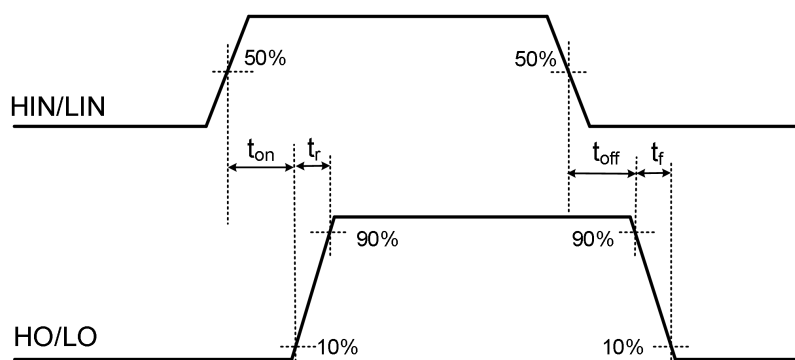
Figure 7 -2 Propagation Time Waveform Definition
