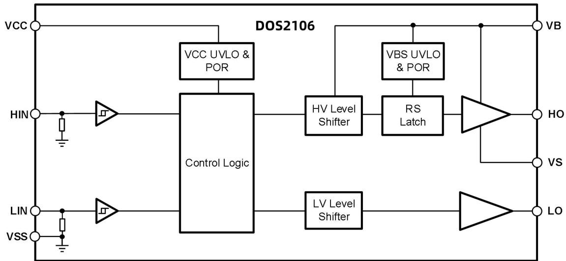
Figure 8-1 Function Block Diagram of DOS2106
