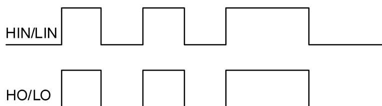
Figure 7 -1 DOS2106 Input and output timing waveform
