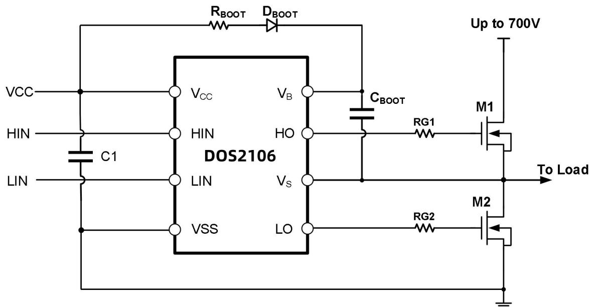
Figure 8-2 Typical application circuit of DOS2106
