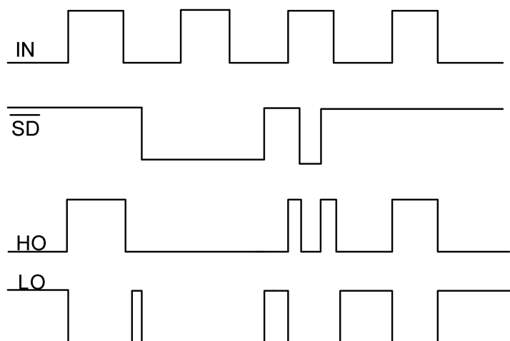
Figure 7-1 DOS2104 Input and output timing waveform
