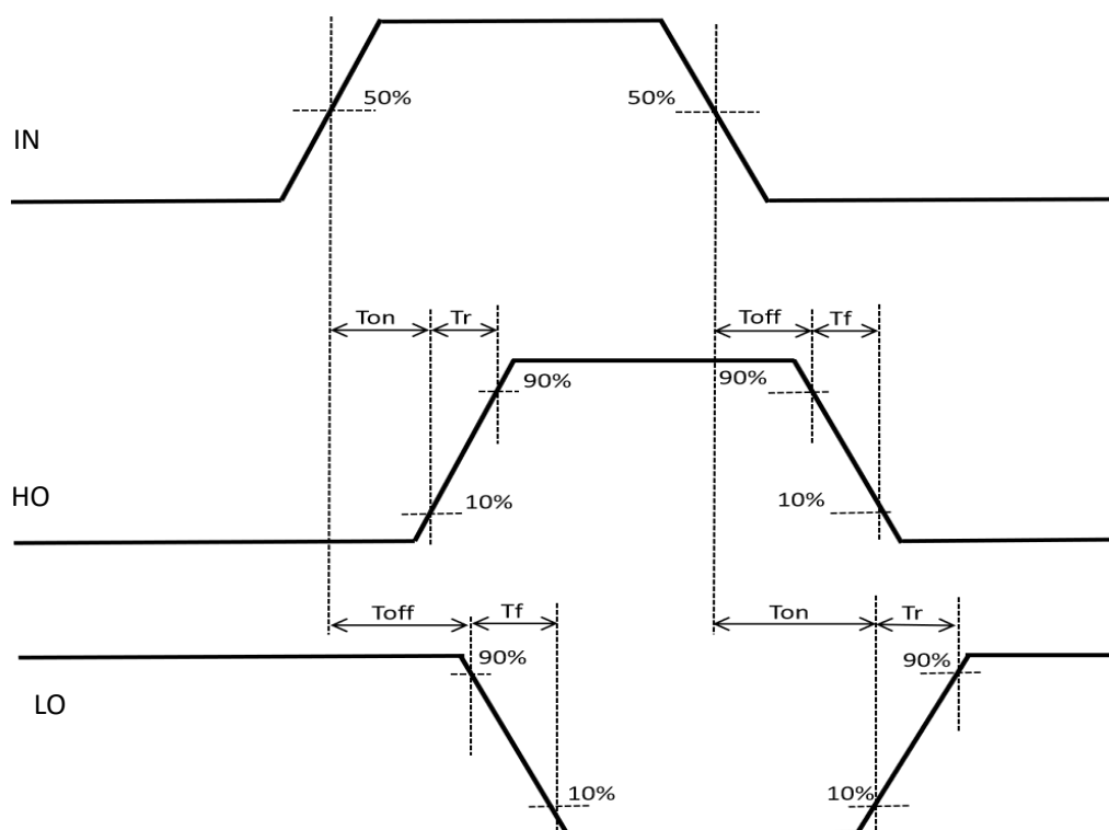
Figure 7-2 Propagation Time Waveform Definition
