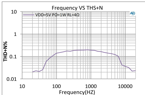
图5：Frequency VS. THD+N
