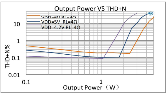
图3 : Output Power VS. THD+N
