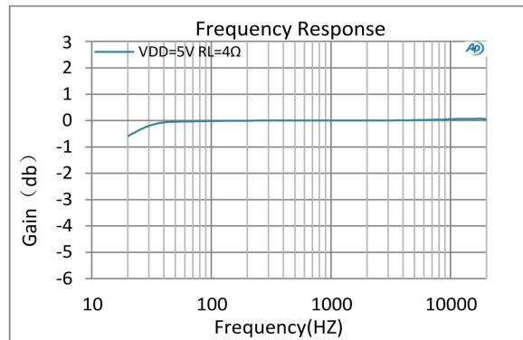
图6：Frequency Response
