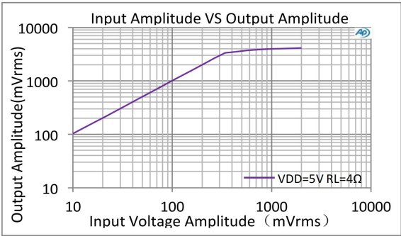
图1 : Input Amplitude VS. OutputPower
