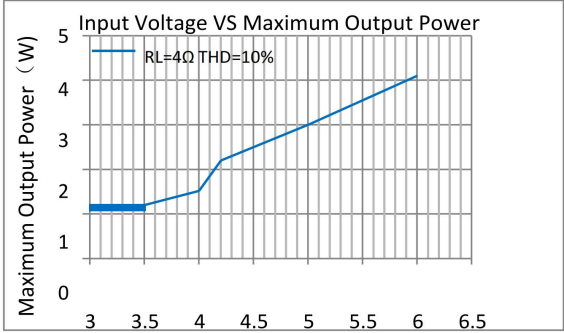
图2 : Input Voltage VS. Output Power
