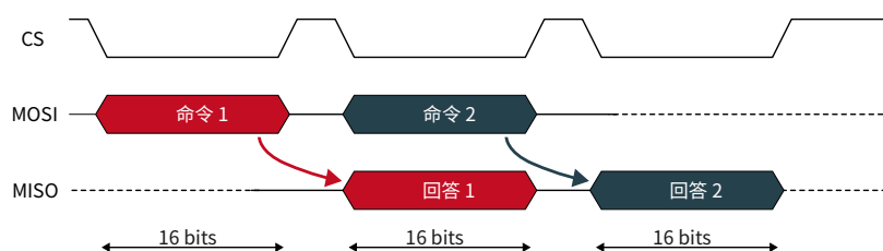
图 8: SPI Command-Response overlapped structure
