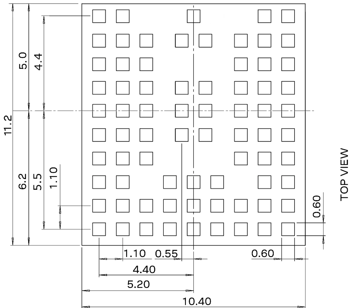
Figure 6: NORA-B2x1 footprint dimension
