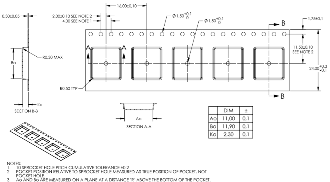
Figure 12 shows the tape and pocket dimensions for NORA-B2x1
