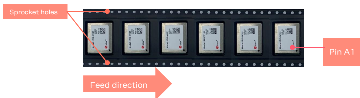
Figure 10: Orientation of IRIS-W101 module on tape
