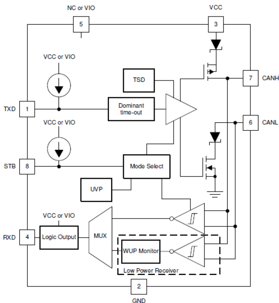
Figure 9. Functional Block Diagram
