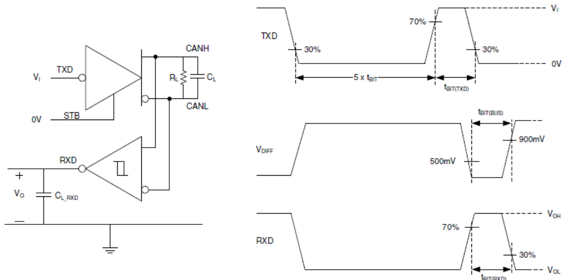
Figure 5. T_{PROP(LOOP)} Test Circuit and Measurement
