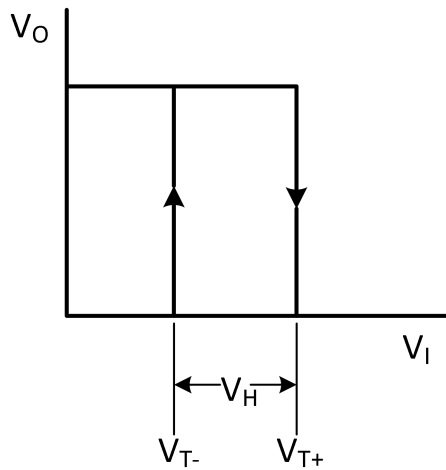
Fig 9. Transfer characteristic
