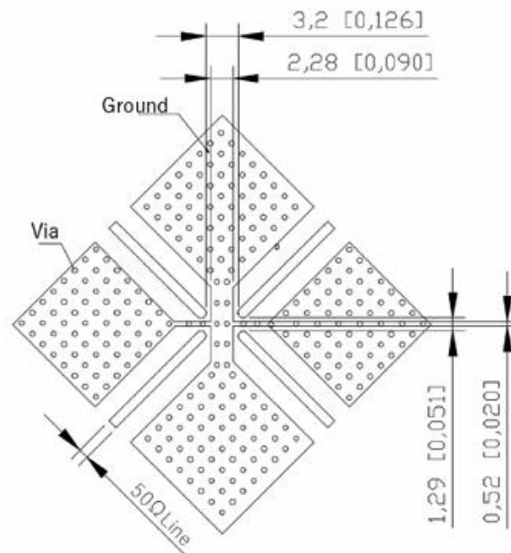
Figure 11. Recommended PCB Layout
