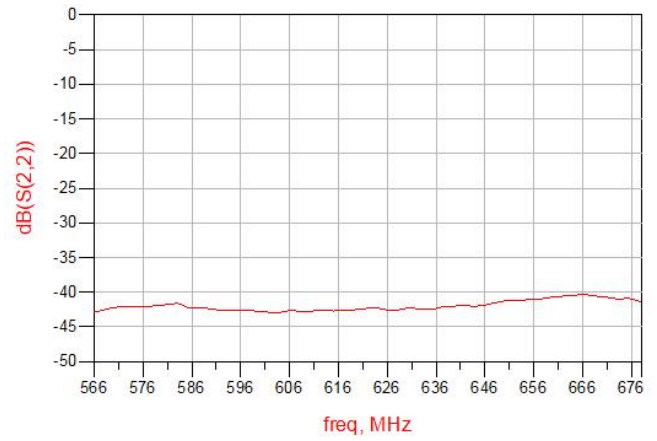
Figure 6. MHC56X30 Return Loss (S22)
