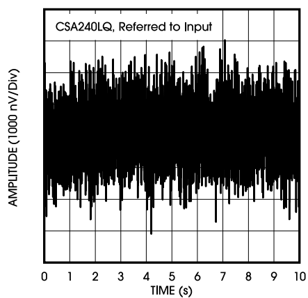
Figure 14. 0.1Hz to 10Hz Voltage Noise
