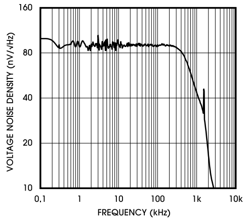
Figure 13. Input-Referred Voltage Noise vs. Frequency
