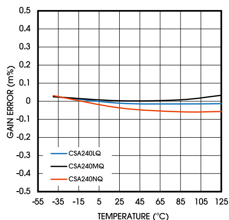
Figure 7. Gain Error vs. Temperature
