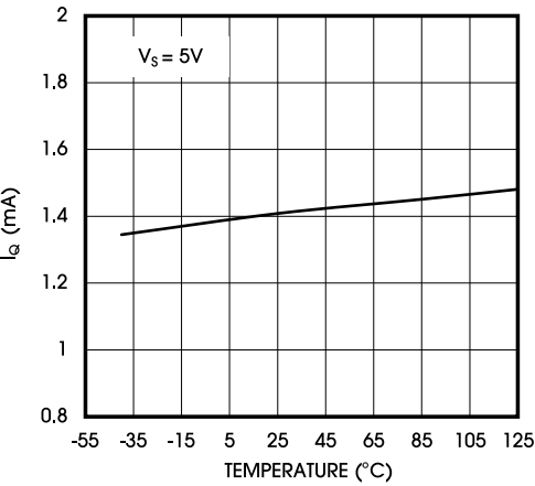
Figure 12. Quiescent Current vs. Temperature
