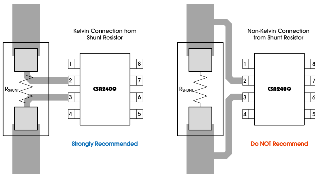
Figure 27. Shunt Connections to the CSA240Q
