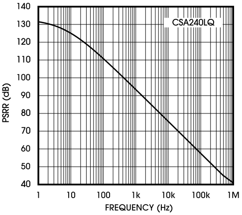
Figure 9. Power-Supply Rejection Ratio vs. Frequency
