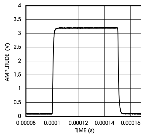
Figure 15. Step Response
