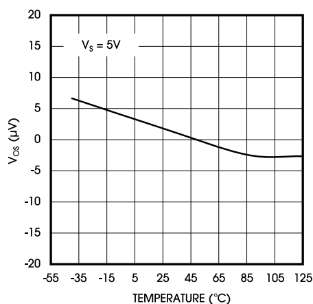
Figure 2. Offset Voltage vs. Temperature
