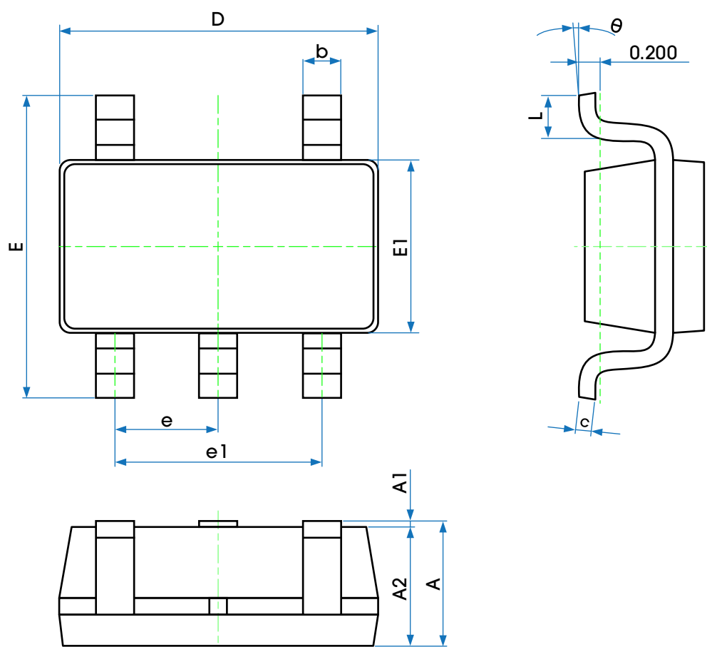
Figure 15. Package View
