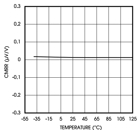
Figure 3. Common-Mode Rejection Ratio vs. Temperature
