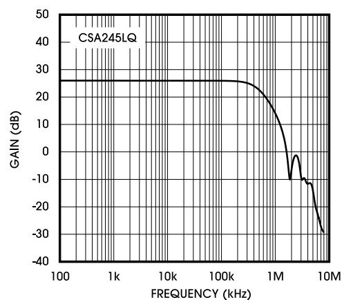
Figure 5. Gain vs. Frequency
