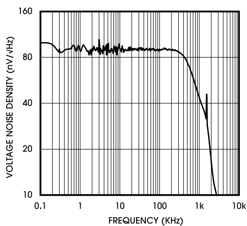
Figure 11. Input-Referred Voltage Noise vs. Frequency
