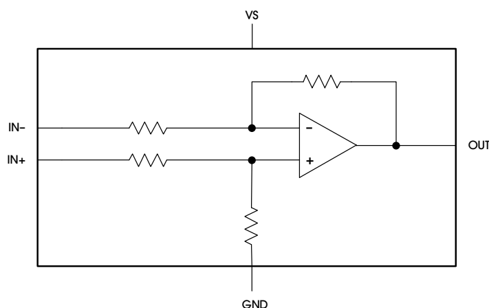
Figure 14. Functional Block Diagram
