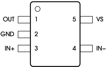
Figure 1. Pin Configuration
