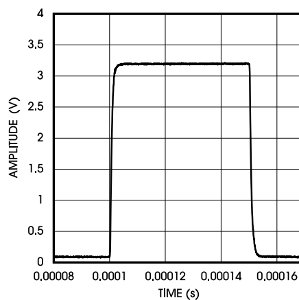
Figure 13. Step Response
