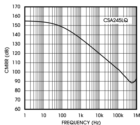
Figure 7. Common-Mode Rejection Ratio vs. Frequency
