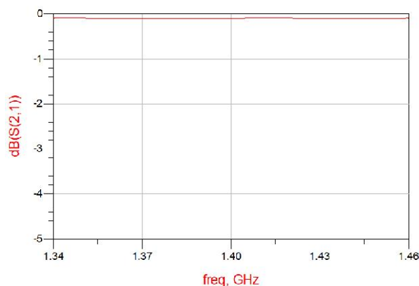
Figure 4. MHC1400M30 Transmission
