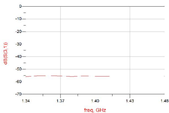
Figure 9. MHC1400M30 Isolation
