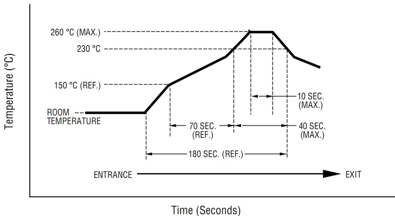
Figure 12. MHC1400M30 Thermal Reflow Profile
