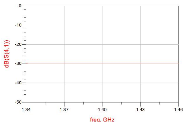
Figure 3. MHC1400M30 Coupling
