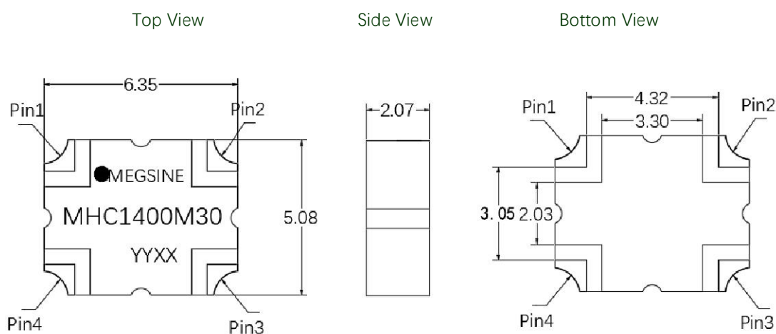
Figure 2. MHC1400M30 Outline Drawing
