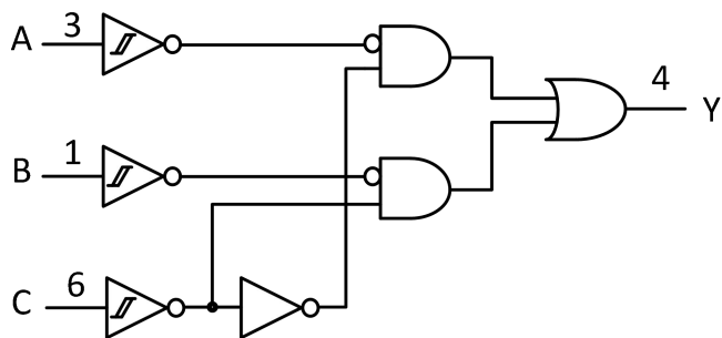
Fig. 1. Logic symbol
