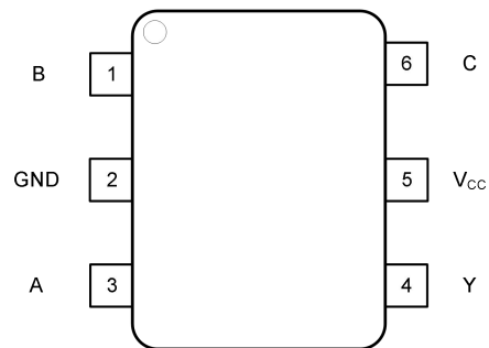
Fig. 2. Top view pin configuration SOT23-6 and SOT363
