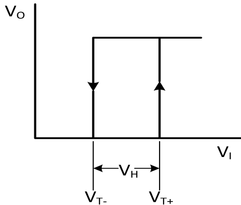
Fig. 14. Transfer characteristic
