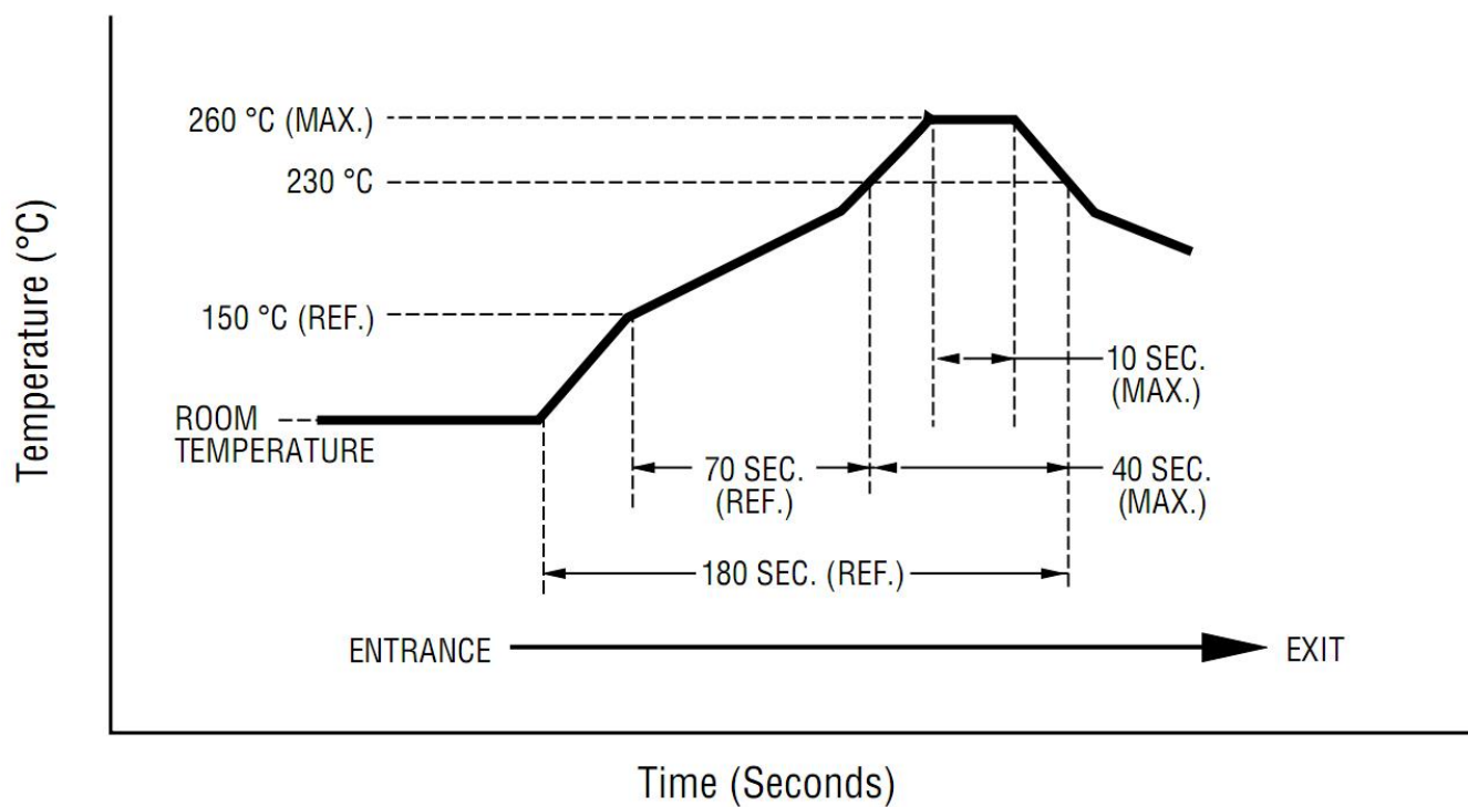
Figure 12. MHC20X30 Thermal Reflow Profile
