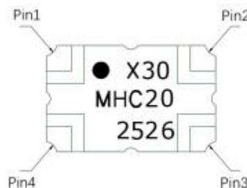
Figure 1. MHC20X30 (Top View)
