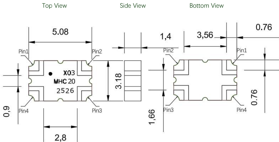
Figure 2. MHC20X30 Outline Drawing
