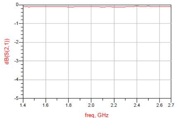
Figure 4. MHC20X30 Transmission
