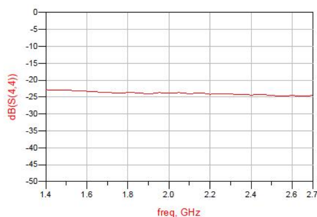
Figure 8. MHC20X30 Return Loss (S44)
