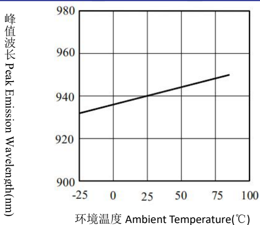
峰值波长与环境温度的关系 Peak Emission Wavelength vs. Ambient Temperature
