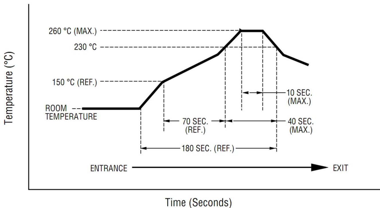
Figure 12. MHC2500M03 Thermal Reflow Profile
