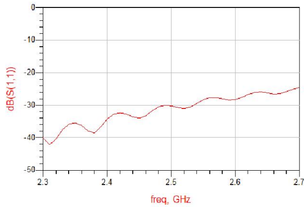
Figure 5. MHC2500M03 Return Loss (S11)
