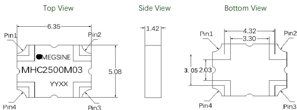
Figure 2. MHC2500M03 Outline Drawing
