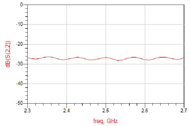
Figure 6. MHC2500M03 Return Loss (S22)
