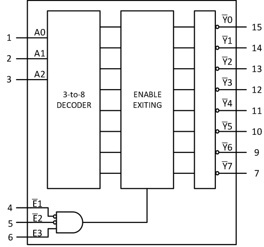
Fig. 2. Functional diagram
