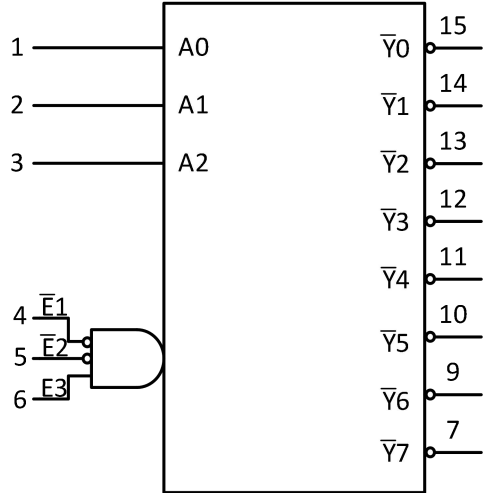
Fig. 1. Logic symbol
