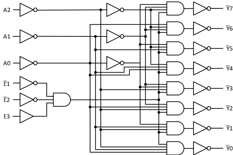
Fig. 3. Logic diagram
