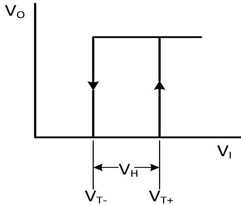
Fig 10. Transfer characteristic
