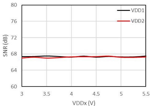
图 3-10 信噪比 vs 供电电压 @ f_{IN} = 10 \text{ kHz}
