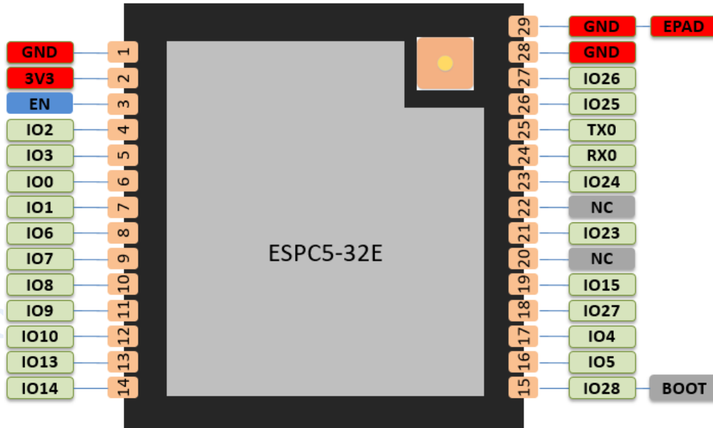
Fig.2.1 ESPC5-32E Pins Definition (Top view)
