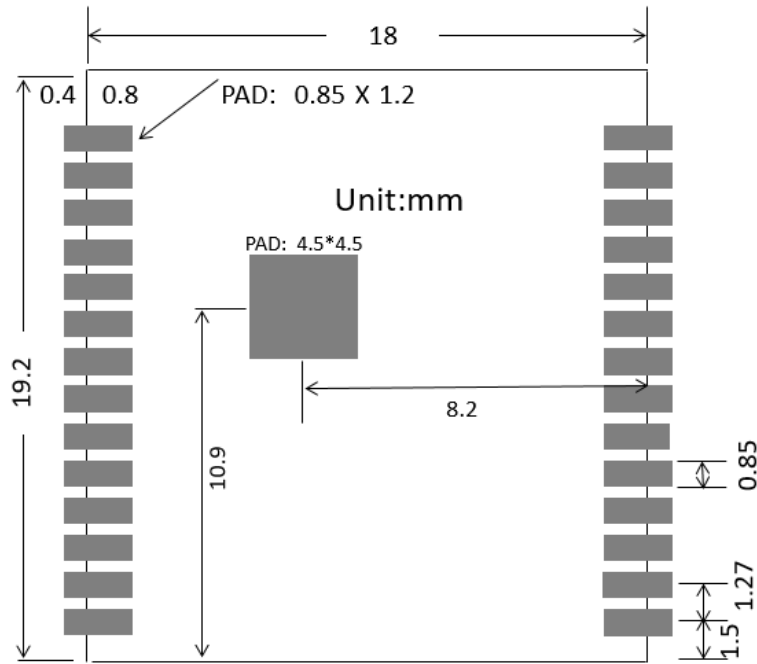
Fig. 3.3 PCB Layout for ESPC5-32E (Top view)
