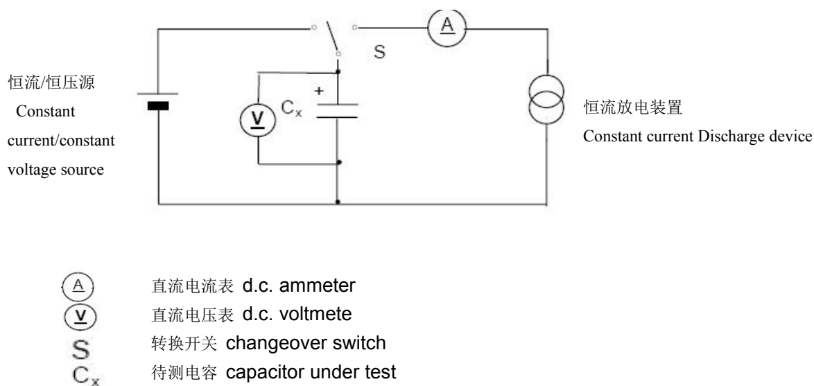
图1 – 恒流放电方法电路 Figure 1 – Circuit for constant current discharge method
