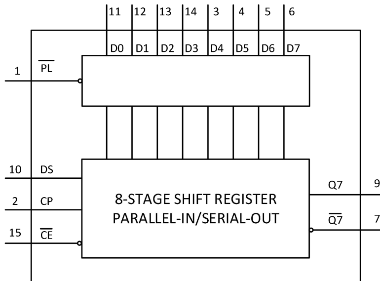
Fig. 3. Logic diagram
