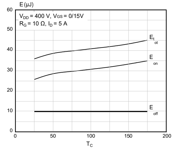
Figure 12. Typical Switching Energy vs. Temperature
